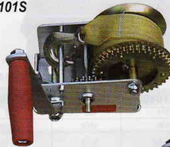
1000 LBS TRT1101S
